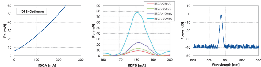
(a) Light output characteristics depending on I_f SOA and I_f DFB
