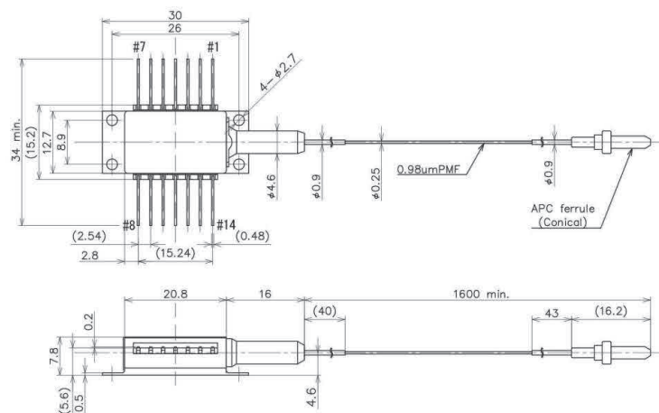
(b) 250um fiber diameter and ferrule type (QLD1x6P-xxC0-11)
