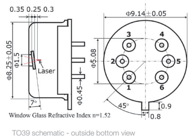
TO39 schematic - outside bottom view
