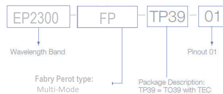
Standard "Pinout 01" option
