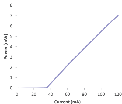
Output power as a function of bias current
