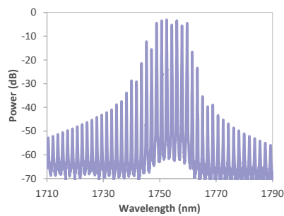
Optical Spectrum at 25°C
