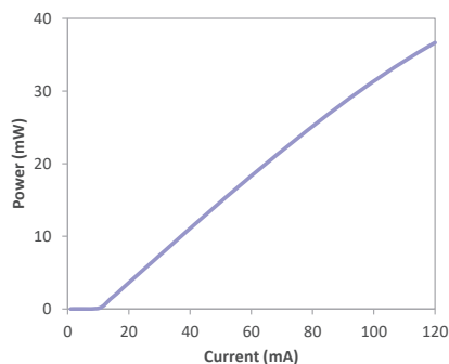
Output power as a function of bias current
