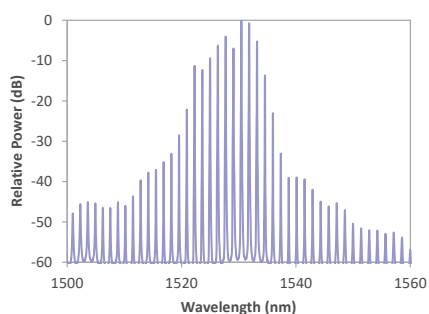
Optical Spectrum at 25°C
