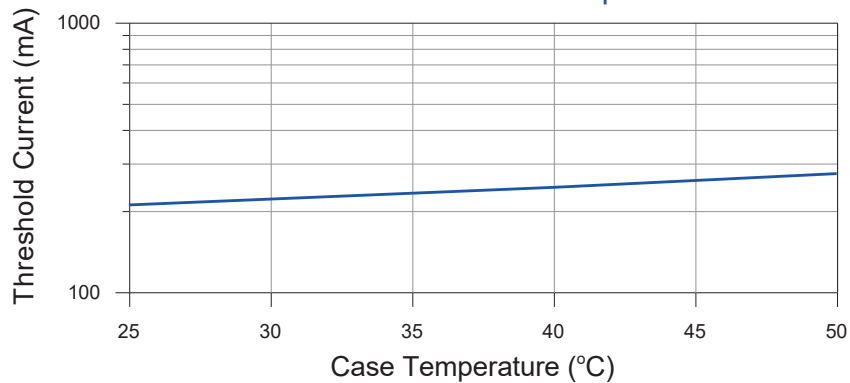
Threshold Current v.s. Case Temperature
