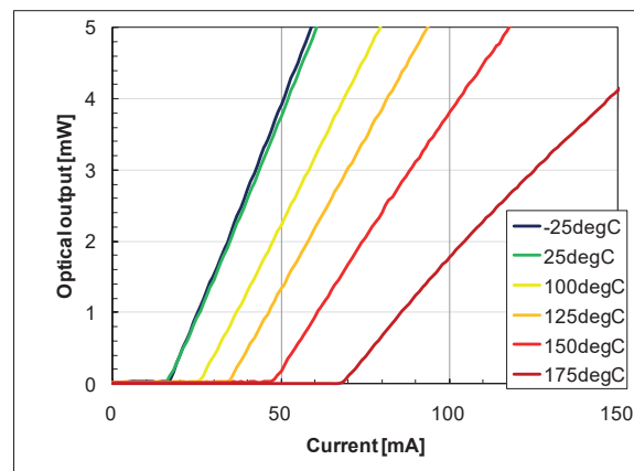
Fig. Typical I-L curve
