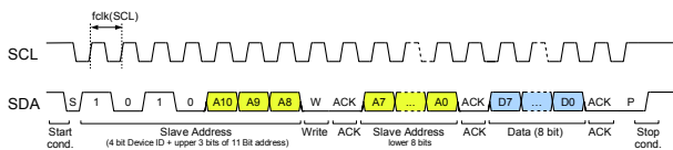
Figure 1: I 2 C slave addressing for writing a single byte to the EEPROM.
