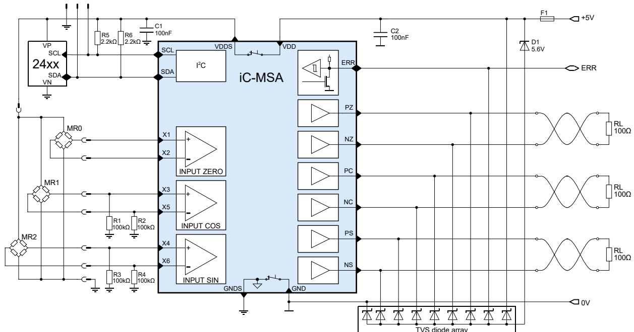
Figure 10: Example circuit for safety-related applications with iC-MSA.
