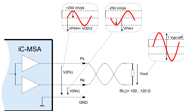
Figure 9: Output amplitude and offset according to Elec. Char. 502 and 503.
