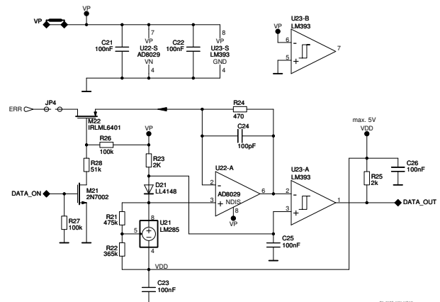
Figure 2: Example circuit for the decoding and conversion of the current-modulated signals to logic levels.
