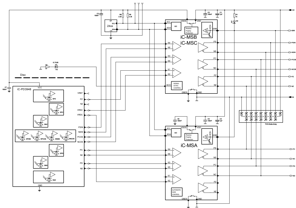
Figure 11: Example circuit with iC-MSA, iC-MSB or iC-MSC, and single EEPROM.
