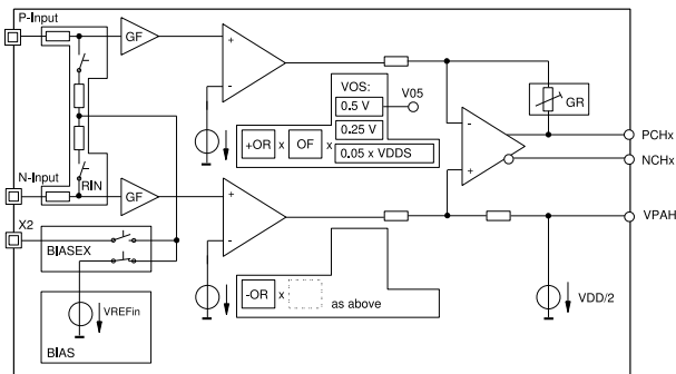
Figure 3: Signal conditioning input circuit.
