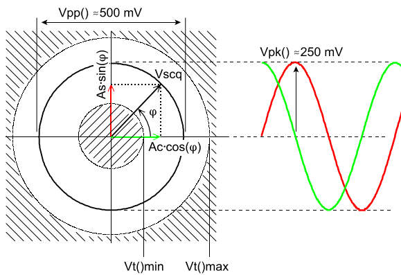
Figure 8: Signal level monitoring with square control (example for AGCOFF = 0, ADJ = 0x32; see Elec. Char. Nos.604 and 605 regarding Vt()min resp. Vt()max).
