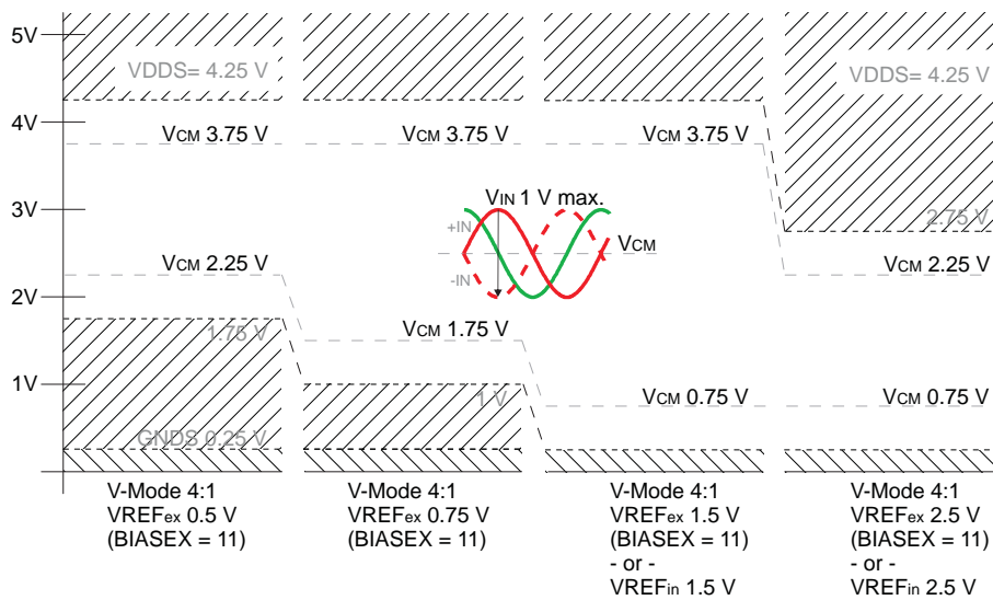
Figure 5: Permissible common mode range for voltage input 4:1 in dependency to the reference voltage.
