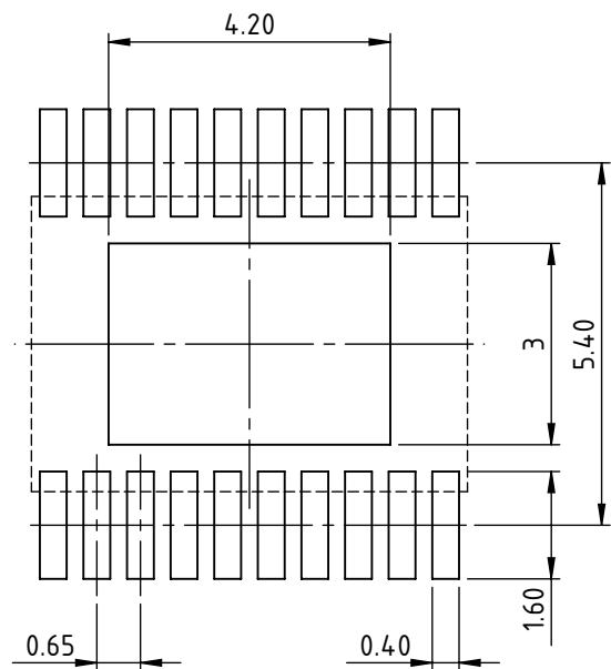
RECOMMENDED PCB-FOOTPRINT
