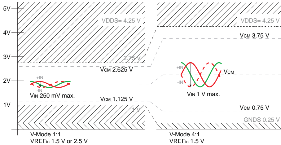
Figure 4: Permissible common mode range and maximum input signal for lowest gain (GR12 = 0x0, GF1, GF2 = 0x00); left side: voltage input 1:1, right side: voltage input 4:1.
