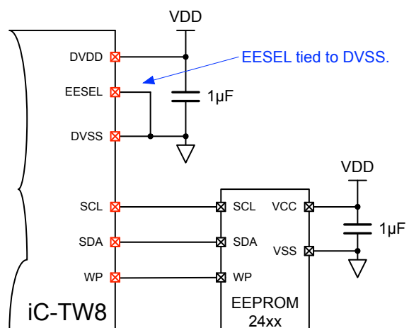
Figure 28: EEPROM Connection
