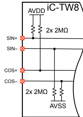
Figure 37: Input Pull-up Resistors
