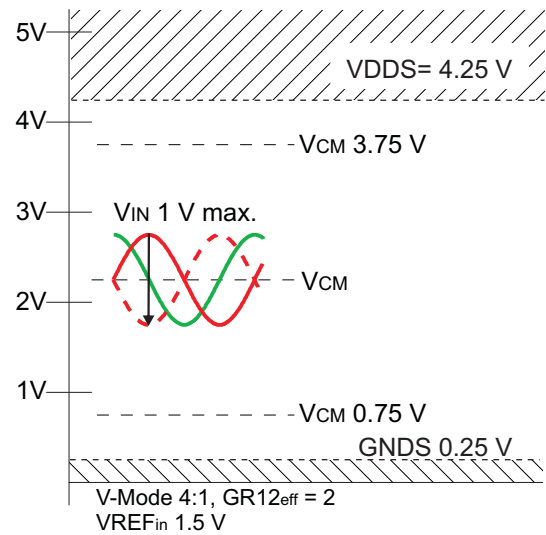
Figure 13: Permissible maximum input amplitude V_{IN} and common mode input range V_{CM} for G_{12_{eff}} = 2.0 and V-Mode 4:1.
