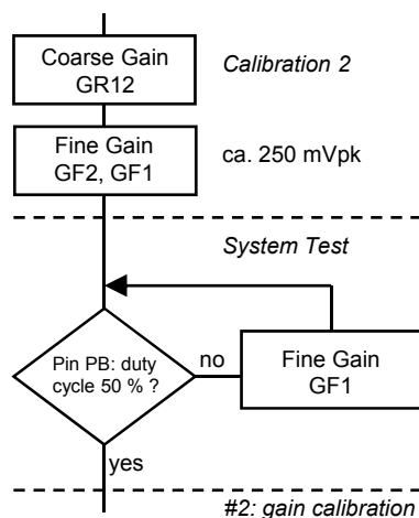
Figure 29: Adjustment of coarse gain GR12 and fine gains GF1 and GF2 to obtain the target amplitude of 250 mVpeak. Amplitude matching is adjusted by fine gain control GF1 of channel CH1.
