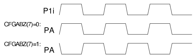
Figure 26: Function of CFGABZ(7)
