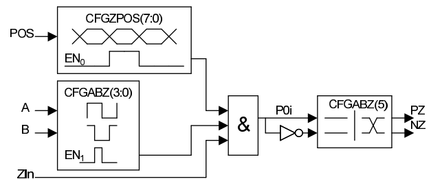
Figure 23: Signal path from Z_{in} to PZ/NZ
