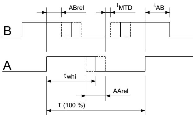
Figure 3: Relative angle error and minimum edge distance.
