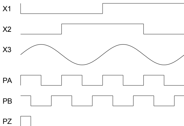
Figure 20: Signal example for interpolation factor x8 (for DUAL = 1).
