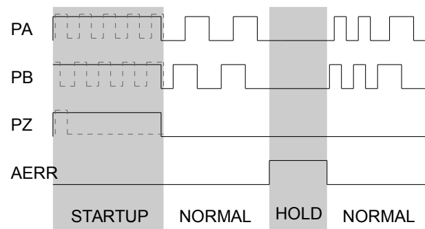
Figure 19: Modes for count signals
