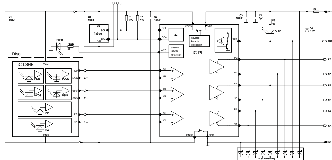
Figure 38: Optical encoder application example.
