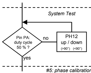
Figure 35: Correction of the sine-to-cosine phase shift by PH12. Repeating the gain and offset calibrations may be reasonable if larger phase correction values are required (refer to chapter signal conditioning for further details).
