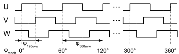
Figure 21: Example of UVW commutation signals.
