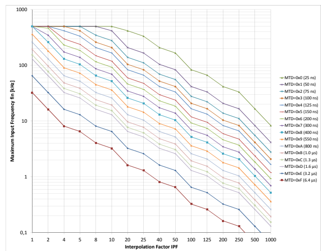
Figure 4: Maximum input frequency depending on interpolation factor. See also Table 43, page 33.
