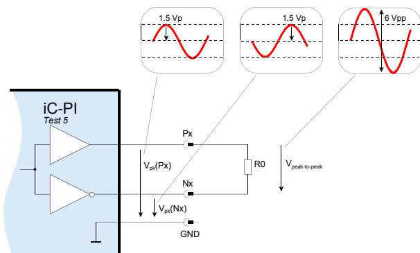
Figure 16: Definition of 6 V pp differential test signal. Termination R0 must be high-impedance (resistive) during all Test and Calibration modes.
