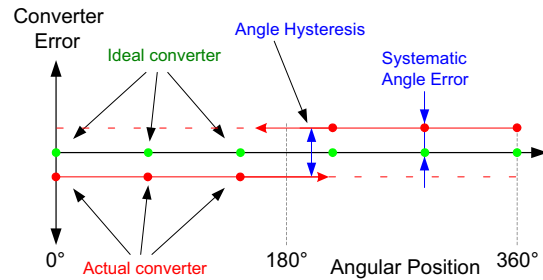
Figure 2: Systematic angle error due to hysteresis.
