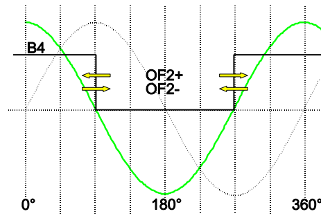
Figure 34: Test signal at pin NB for offset calibration of channel CH2. The adjustment is ideal at a duty ratio of 50%.
