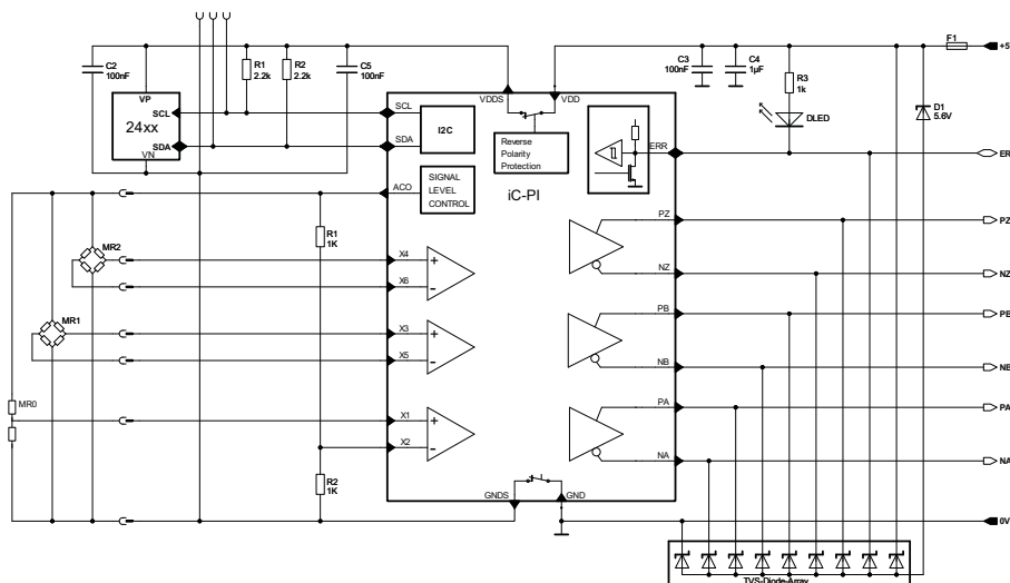
Figure 39: Magnetic encoder application example.
