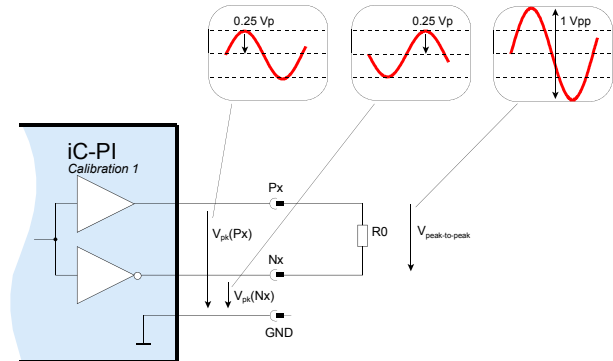
Figure 17: Definition of 1 Vpp differential test signal. Note that the outputs should not be loaded during Test and Calibration modes ( R0 must be high resistance).
