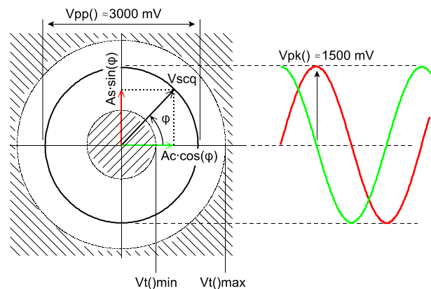
Figure 18: Signal monitoring and test signals in Test 5 mode (example for ACOS(4:0) = 0x19).
