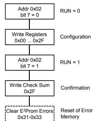
Figure 9: Programming via I 2 C. RUN is altered by changing only bit 7 of address 0x02 and leaving bits 6:0 unchanged.
