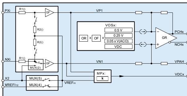
Figure 11: Signal conditioning input circuit.
