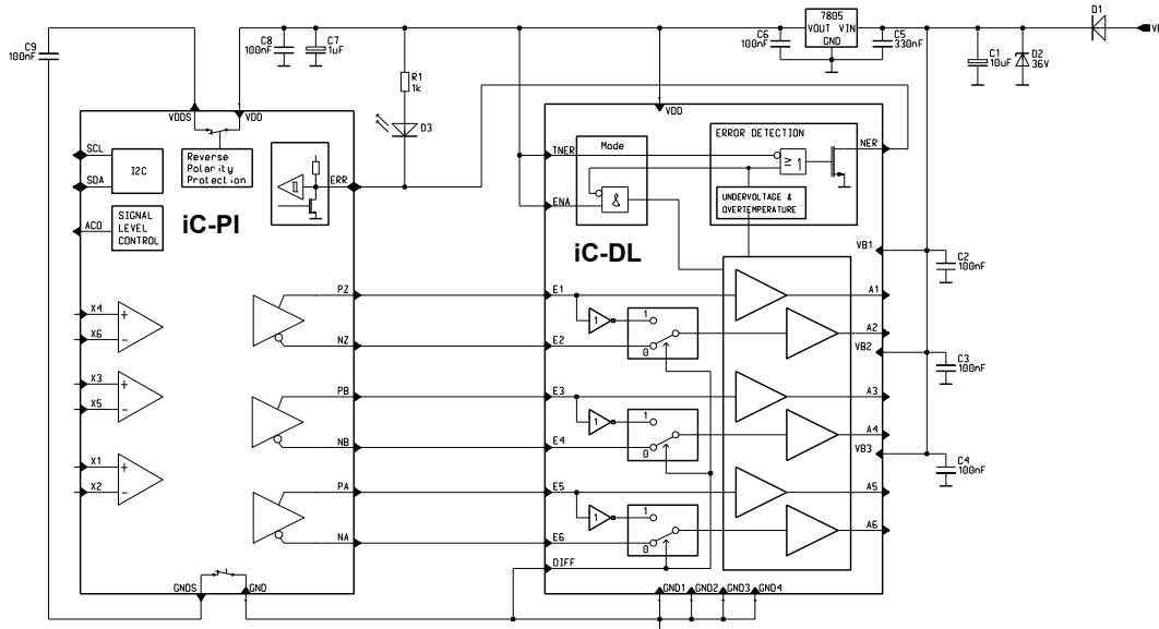
Figure 40: Application example with 24 V line driver.
