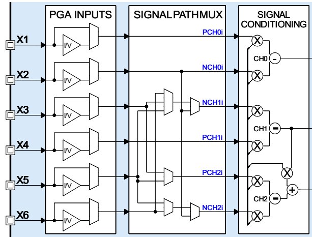
Figure 15: Signal Path Multiplexer
