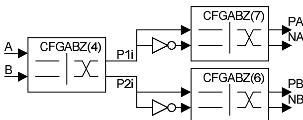
Figure 22: Signal path from A and B to PA/NA and PB/NB
