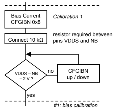
Figure 28: Verification of the bias current is recommended, and if necessary adjustment (see chapter bias current source).
