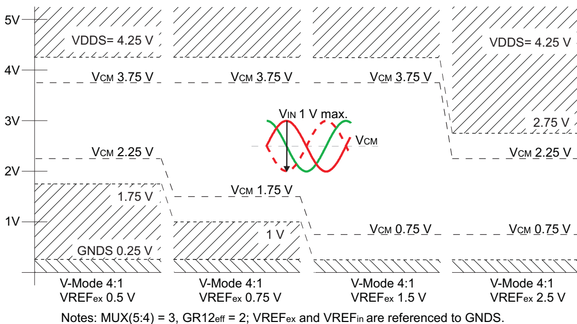
Figure 14: Permissible maximum input amplitude V_{IN} and common mode input range V_{CM} for G_{12_{eff}} = 2.0 and V-Mode 4:1 in dependency to the reference voltage.
