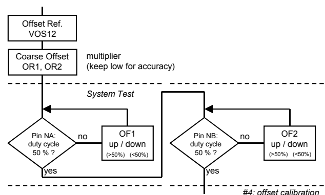
Figure 32: Selection of coarse offset OR1 and OR2 and the subsequent calibration of OF1 and OF2. Selecting OR1 and OR2 as small as possible permits a finer adjustment.
