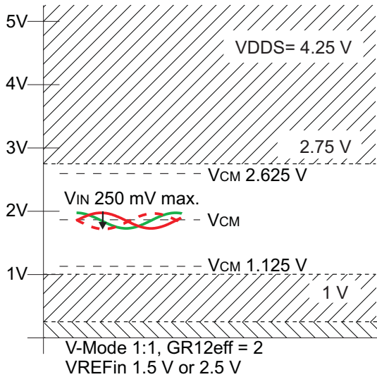
Figure 12: Permissible maximum input amplitude V_{IN} and common mode input range V_{CM} for G_{12_{eff}} = 2.0 and V-Mode 1:1
