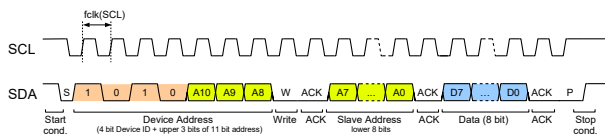
Figure 5: I 2 C slave addressing for writing a single byte to the EEPROM.
