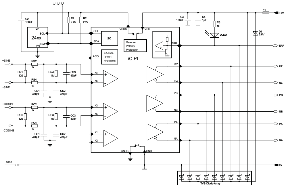
Figure 41: Input circuit for sine encoders (0.8 Vpp to 1.2 Vpp) with 120 Ω termination and low-pass filtering. RS2/RS4 and RC2/RC4 serve as protection against ESD and transients. RS3 and RC3 reduce the input signal levels to 1/3 suiting for an overall gain of 18 (GR12 x GF1, resp. G12 x GF2).
