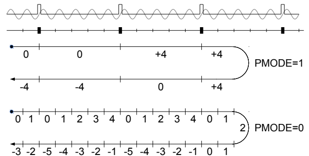
Figure 10: Output of PERIOD register in PDMODE 0 and 1 with index pulse every 5 periods
