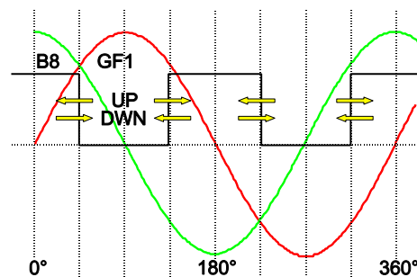
Figure 30: Test signal at pin PB for fine tuning of channel CH1 for identical amplitudes. The adjustment is ideal at a duty ratio of 50%.
