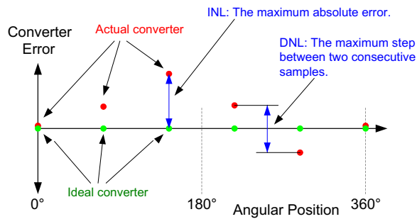
Figure 1: Integral and differential nonlinearity.
