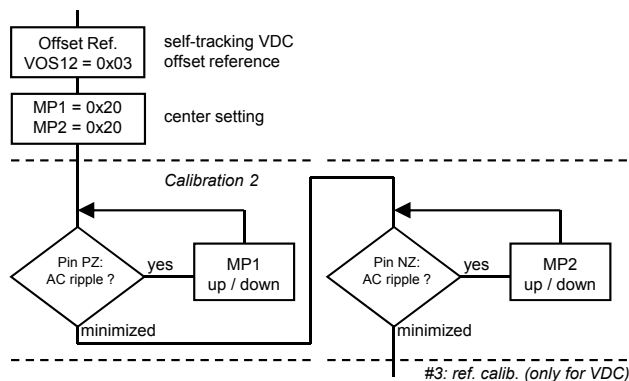
Figure 31: When using the self-tracking VDC offset references, an adjustment of the VDC center potentials for minimal AC ripple is advisable. Other offset references do not require this adjustment.
