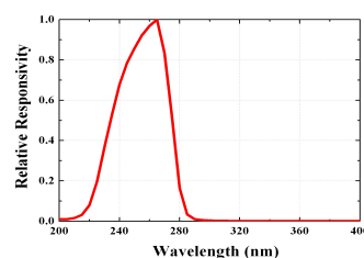
Fig. 2 Responsivity Curve
